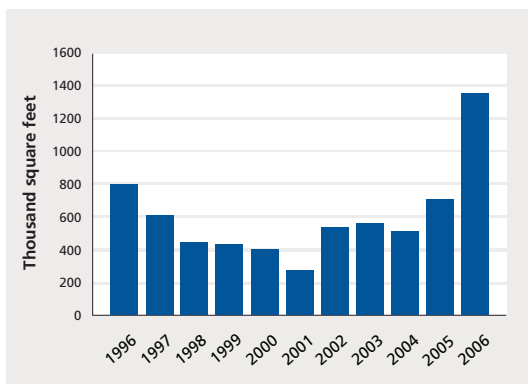
FIGURE 15 U.S. shipments of medium temperature solar thermal panels, 1996-2006 m
