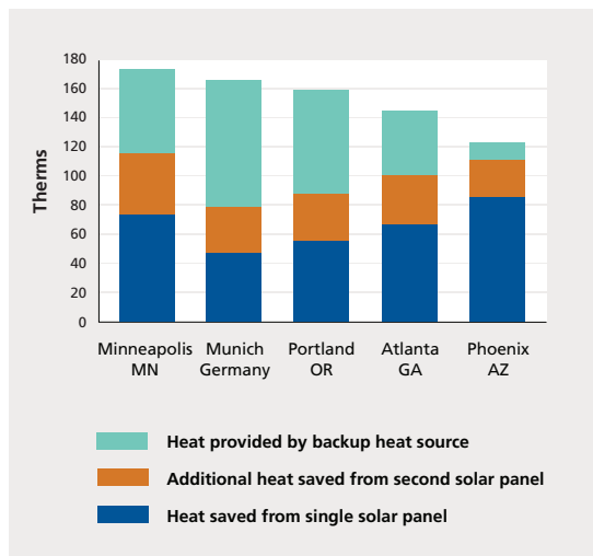
FIGURE 2 Solar output for one and two panel solar hot water systems in five major cities b
