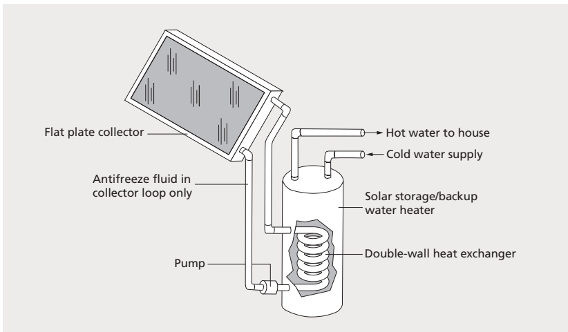
FIGURE 5 Active, closed-loop solar water heater e
