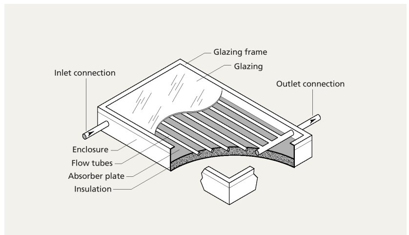
FIGURE 6 Flat plate collector 1
