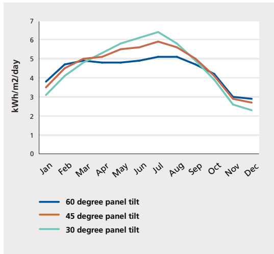
FIGURE 4 Average monthly solar resource for Minneapolis at various panel tilt angles (kWh/m 2 /day) d
